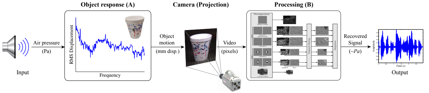
Figure 3: We model the visual microphone as a system that operates on sound. Component A (Section 5.1) models an object’s response to sound, and is purely physical—taking as input changes in air pressure, measured in Pascals, and producing physical displacement of the object over time, measured in millimeters. The response of the object to the sound depends on various factors such as the sound level at the object, and the object’s material and shape. A camera then records the object, transforming the physical displacements into pixel motions in a video. Component B (Section 3, Section 5.2) is our spatiotemporal processing pipeline, which transforms the motions in the video back into sound. The resulting 1D signal is unit-less, but is correlated with the input Pascals and can therefore be played and analyzed as sound.
